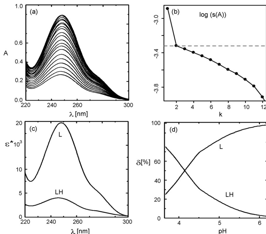
Fig. 4. The nonlinear regression analysis of the protonation equilibria model and factor analysis of flurbiprofen: (a) absorption spectra in dependence on pH at 25 °C, (b) Cattel's scree plot of the Wernimont–Kankare procedure for determination of the number of light-absorbing species in the mixture k^*=2 leads to the actual instrumental error of the spectrophotometer used s_{\text{inst}}(A)=0.48 mAU (INDICES in S-Plus), (c) pure spectra profiles of molar absorptivities vs. wavelengths for species L and LH and (d) distribution diagram of the relative concentrations of species L and LH of flurbiprofen in dependence on pH at 25 °C (SPECFIT, SQUAD and ORIGIN).
